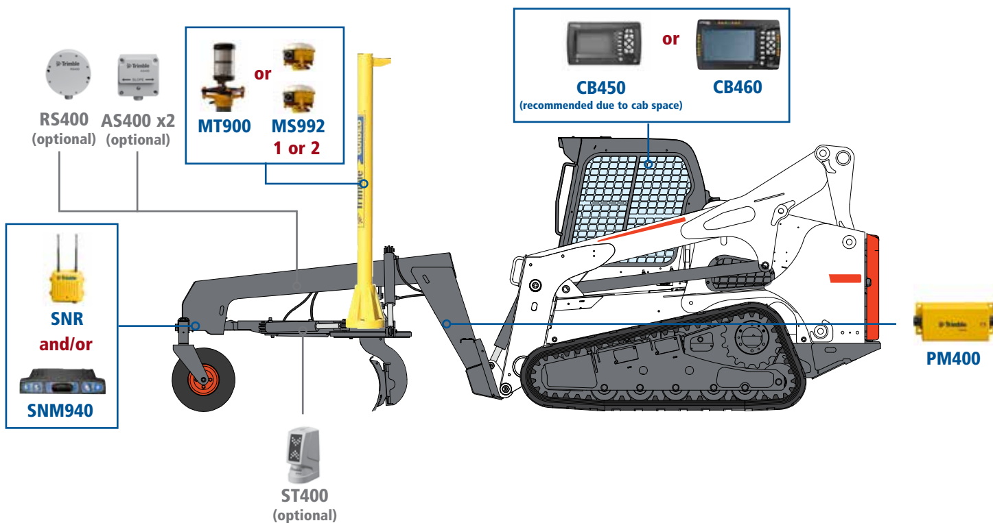
Bobcat HD Grader Attachment System Configuration
