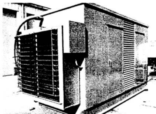
This standby gen set for sewer pump back-up has a load bank built into its enclosure. The gen set fan cools both the radiator and the load bank. Load testing doesn't interfere with the on-site electrical system.
